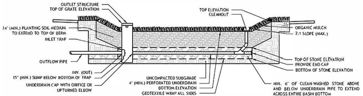
Figure 5: Example Underdrain Detail (courtesy of Philadelphia Water Department's Stormwater Management Guidance Design Manual)
