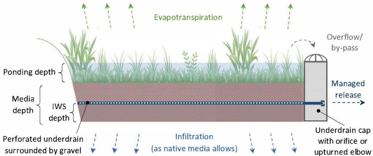
Figure 6: Managed Release Concept with Capped / Orifice Underdrain with Maintenance Access for a Vegetated BMP
